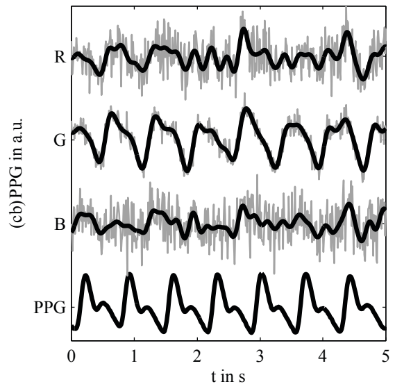
Fig. 2. Sample cbPPG excerpt showing signals extracted from one ROI on patients face for three color channels R,G,B (grey: cbPPG_{n,color} signals, black: lowpass (5 Hz) filtered signals) with corresponding reference PPG.
